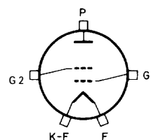
Figure 8 - Terminal Diagram
