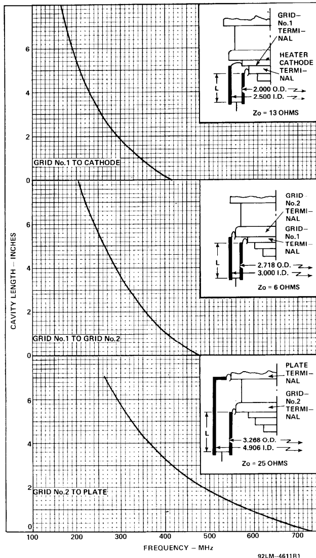
Figure 6 - Tuning Characteristics
