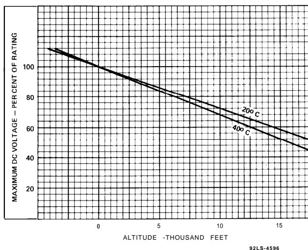
Figure 1 - Maximum DC Voltage vs Altitude
